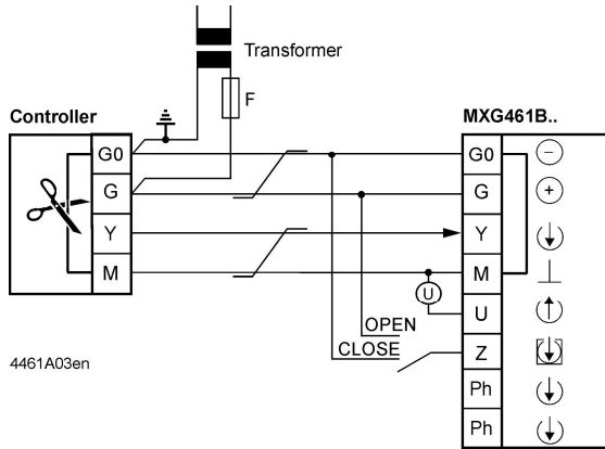
Common Transformer
