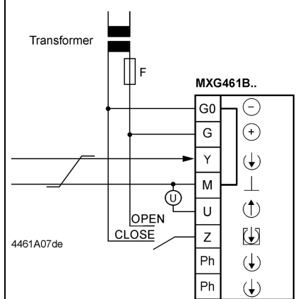
Separate Transformer
