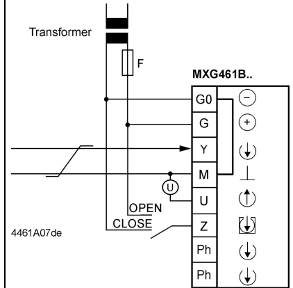
Separate Transformer
