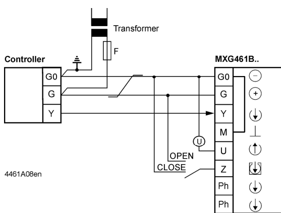
Common Transformer
