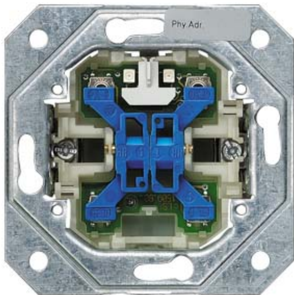
INSTABUS EIB DELTA BUS COUPLING UNIT FM 116 W/O AST, CENTER POSITION 2FOLD
