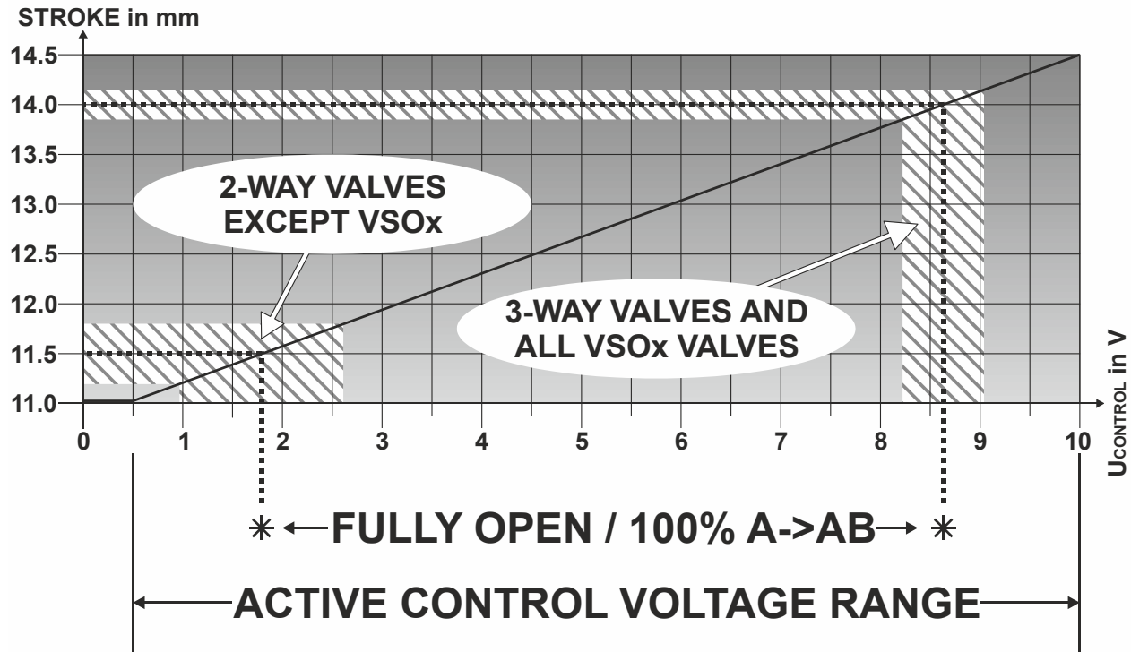
Fig. 10. Characteristic (stroke vs. voltage)
